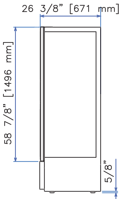
UCRR(F)-17 Side View
