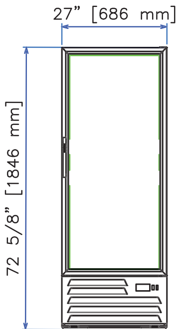
UCRR(F)-17 Front View
