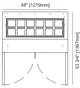
APTS-48-12 Front
