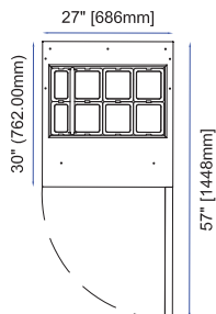
APTS-27-8 Front
