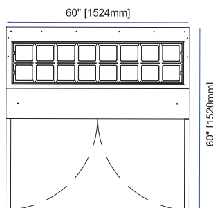
APTS-60-16 Front
