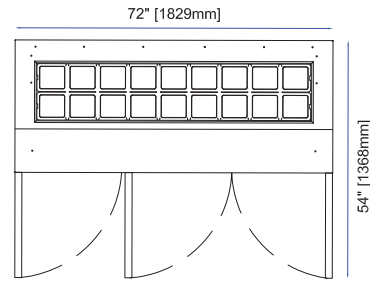
APTS-72-18 Front
