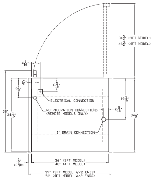
PLAN VIEW (3' & 4')
