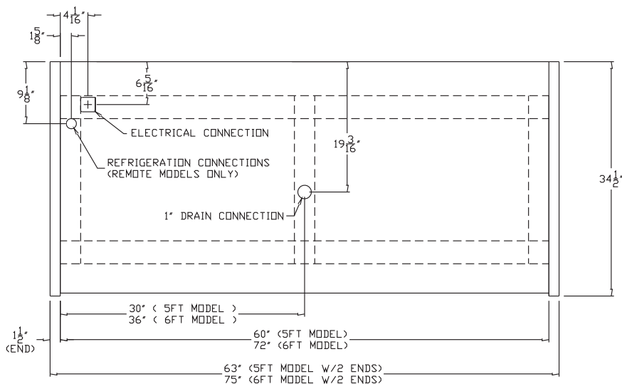
PLAN VIEW (5' & 6')
