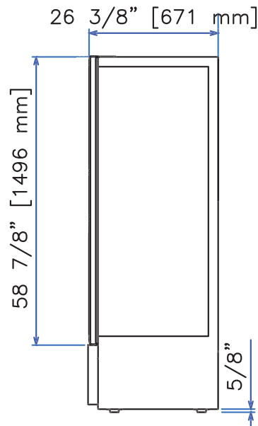
ARR(F)-17 Side
