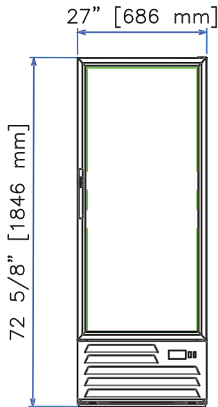
ARR(F)-17 Front
