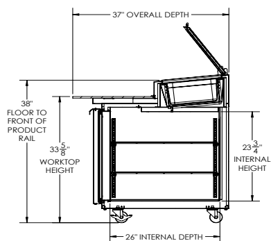
ELEVATION VIEW
