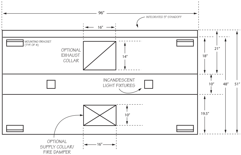
BSSM48-8 PLAN VIEW DETAIL
