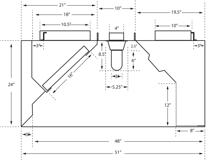
BSSM48-8 PROFILE VIEW DETAIL
