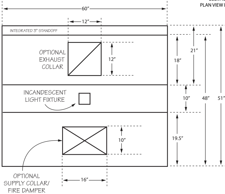
BSSM48-5 PLAN VIEW DETAIL
