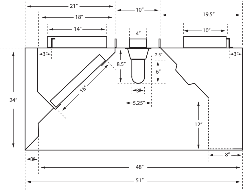
BSSM48-11 PROFILE VIEW DETAIL
