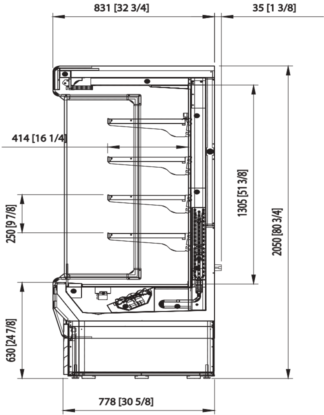
Side view
