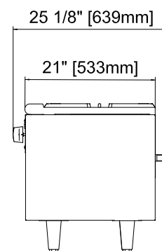
• AESP 18/48 common side view
